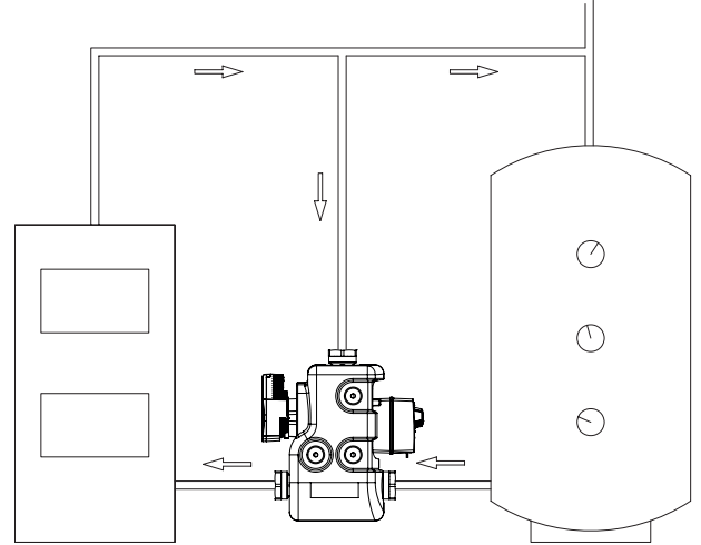
BOILER CAPACITY DIAGRAM
